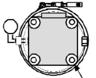
6.30-in. sq. pad w/4 holes 1/8-in. Ø on 7-in. bolt circle
