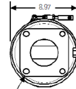
6.30-in. sq. flange w/4 blind holes tapped 1/2-in.-13 UNC on 7-in. bolt circle
